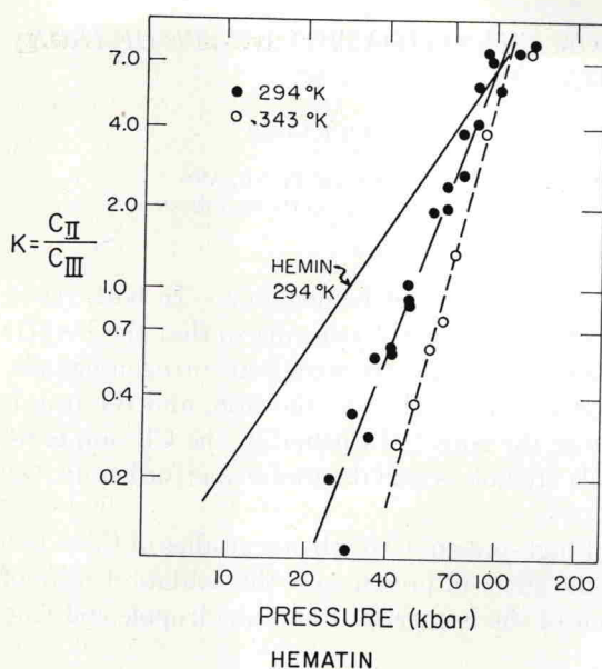
FIG. 2.— \ln K vs. \ln P in hematin.
